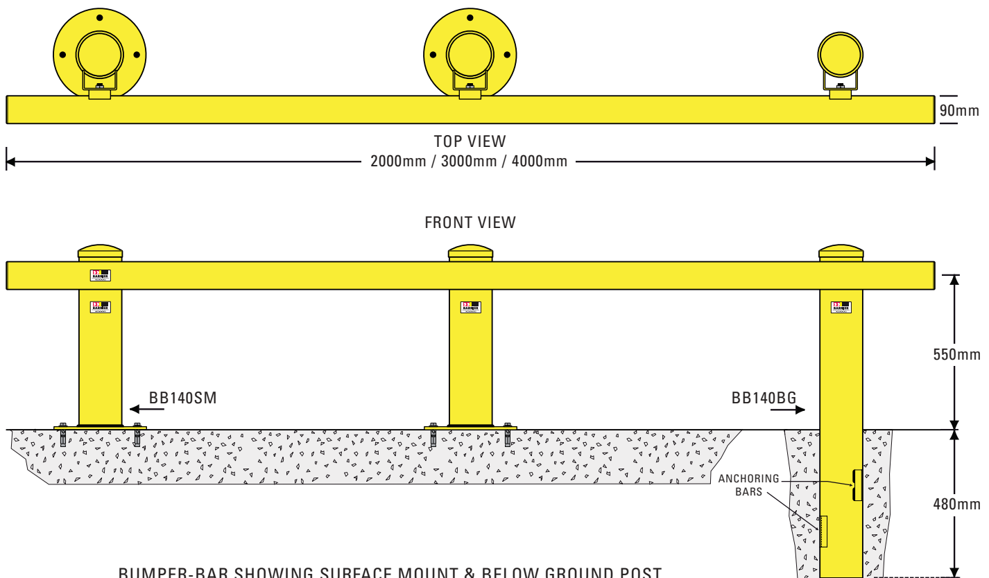
BUMPER-BAR SHOWING SURFACE MOUNT & BELOW GROUND POST
