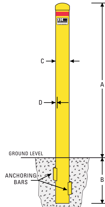
BELOW-GROUND MODEL
